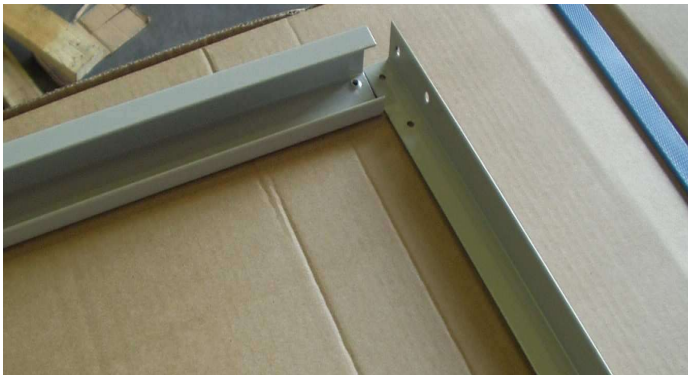
STEP 3: ASSEMBLE THE FIX END OF THE SHORT MEMBER WITH LONG MEMBER USING SCREW
